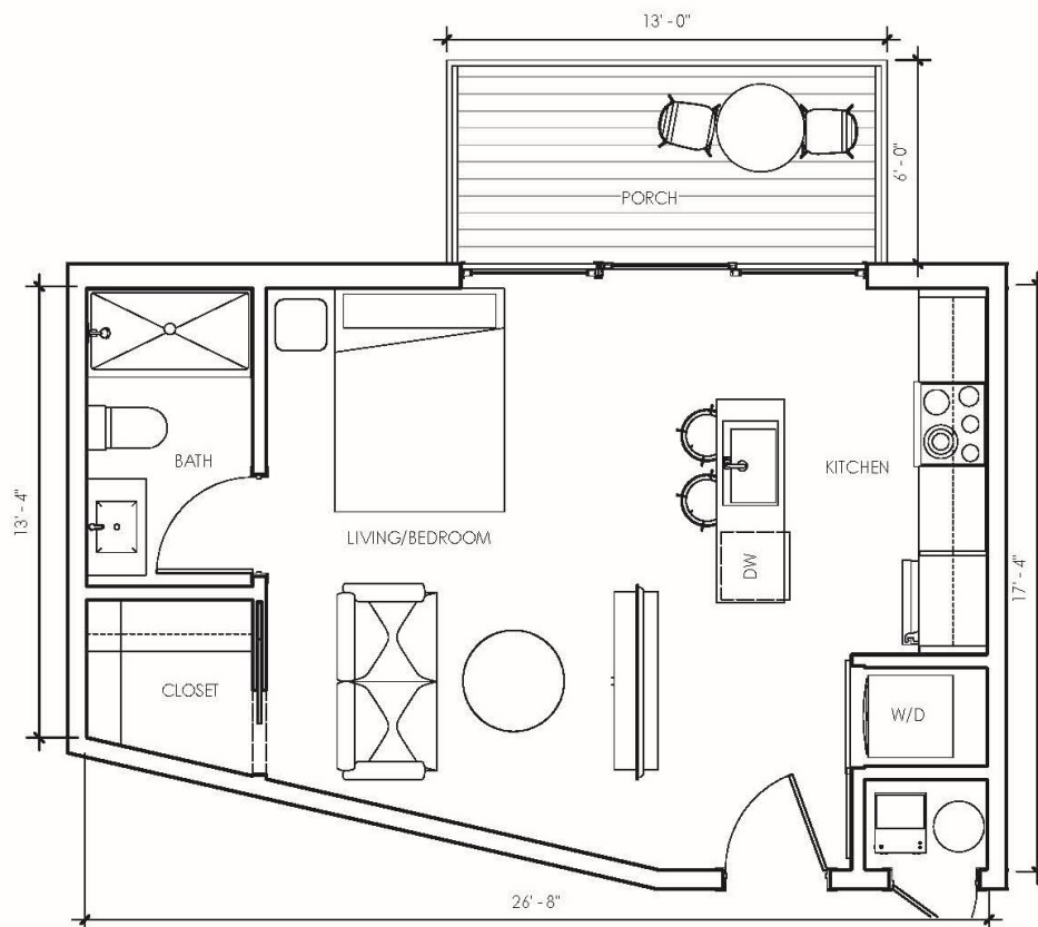
UNIT TYPE A-003 - STUDIO A-103, A-203, A-303, A-403, A-503 443 SF
